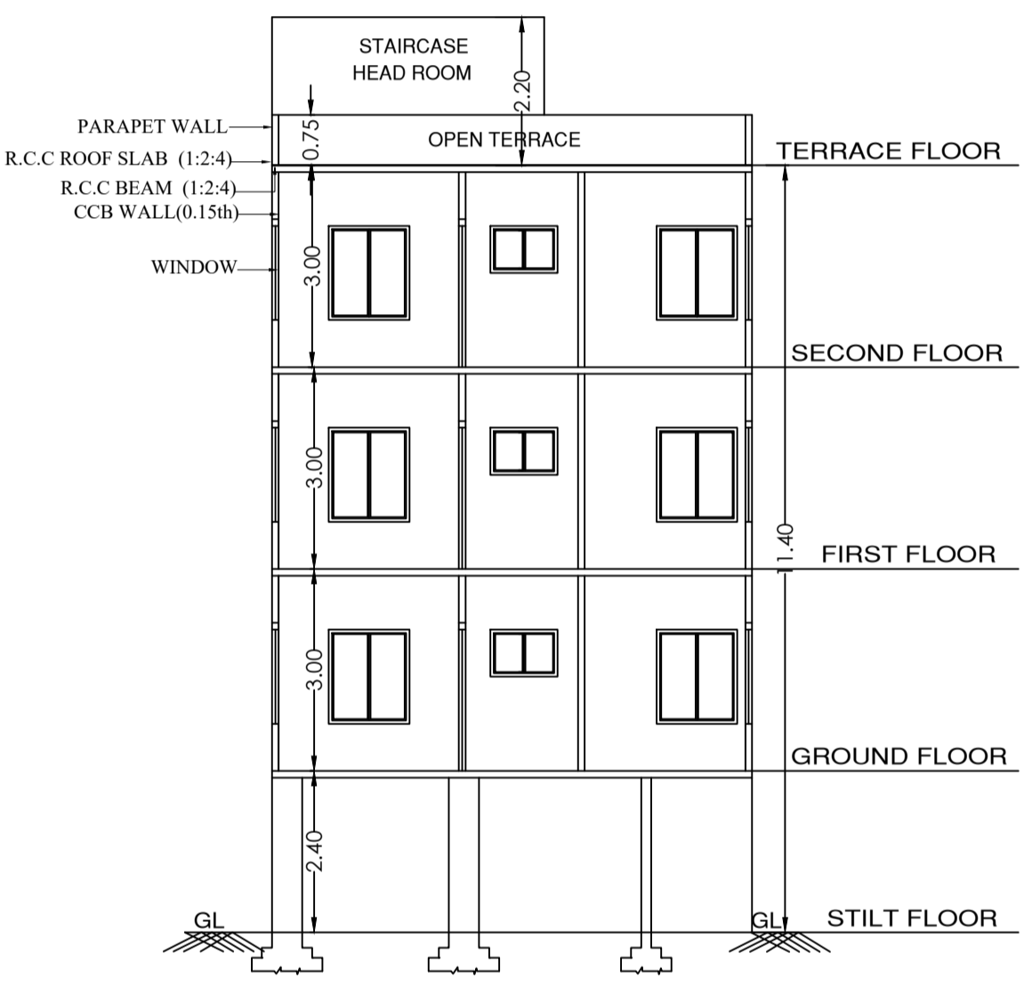
SCETION @ 'A'-'A'
